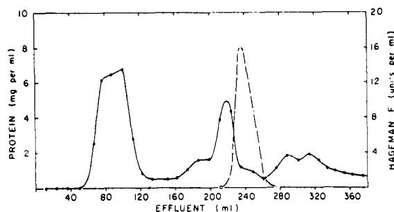
FIG. 2.—The chromatography of activated Hageman factor on a 2 × 22 cm DEAE column. Protein was eluted from the column by a buffer gradient between 0.025 M barbital buffer, pH 7.45, and 0.025 M barbital buffer-0.25 M NaCl, pH 7.45; ●—● refers to protein; O---O refers to Hageman factor activity. See text for details.
